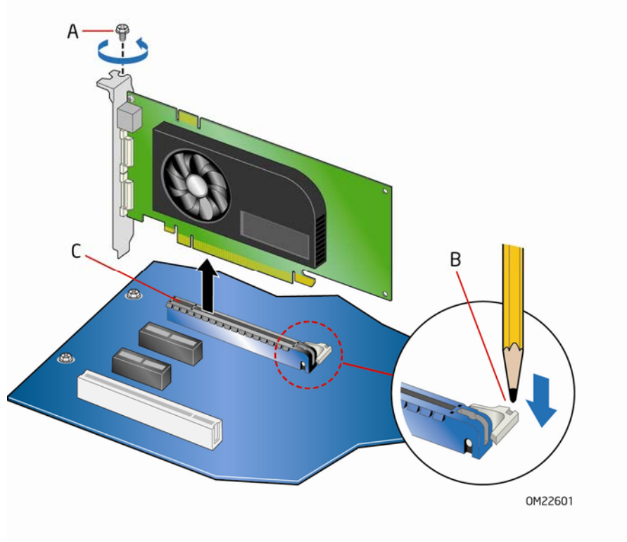
Figure 18. Removing a PCI Express x16 Graphics Card
