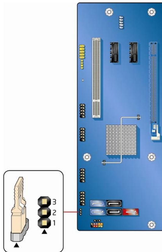
Figure 24. Location of the BIOS Configuration Jumper Block
